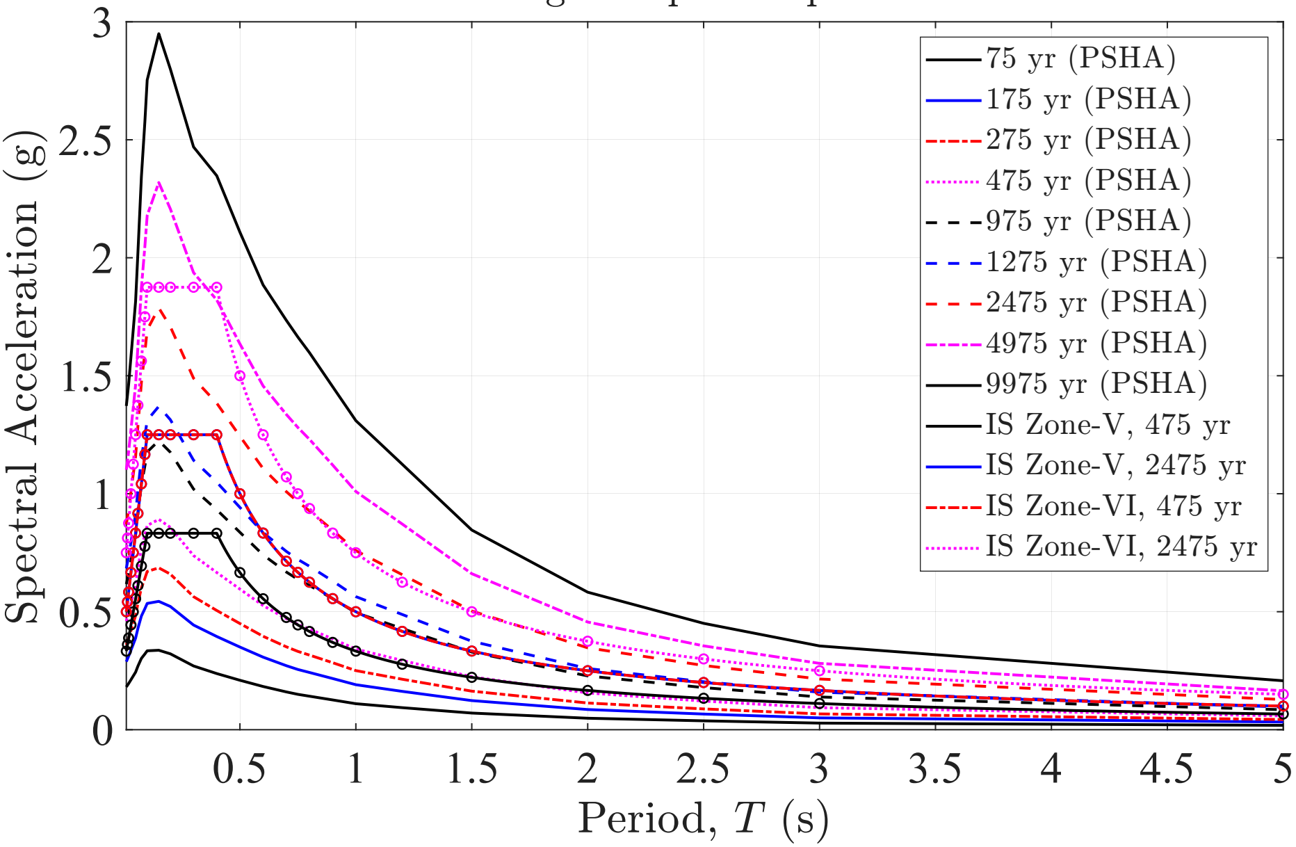
UHS and IS Design Response Spectrum - Guwahati
